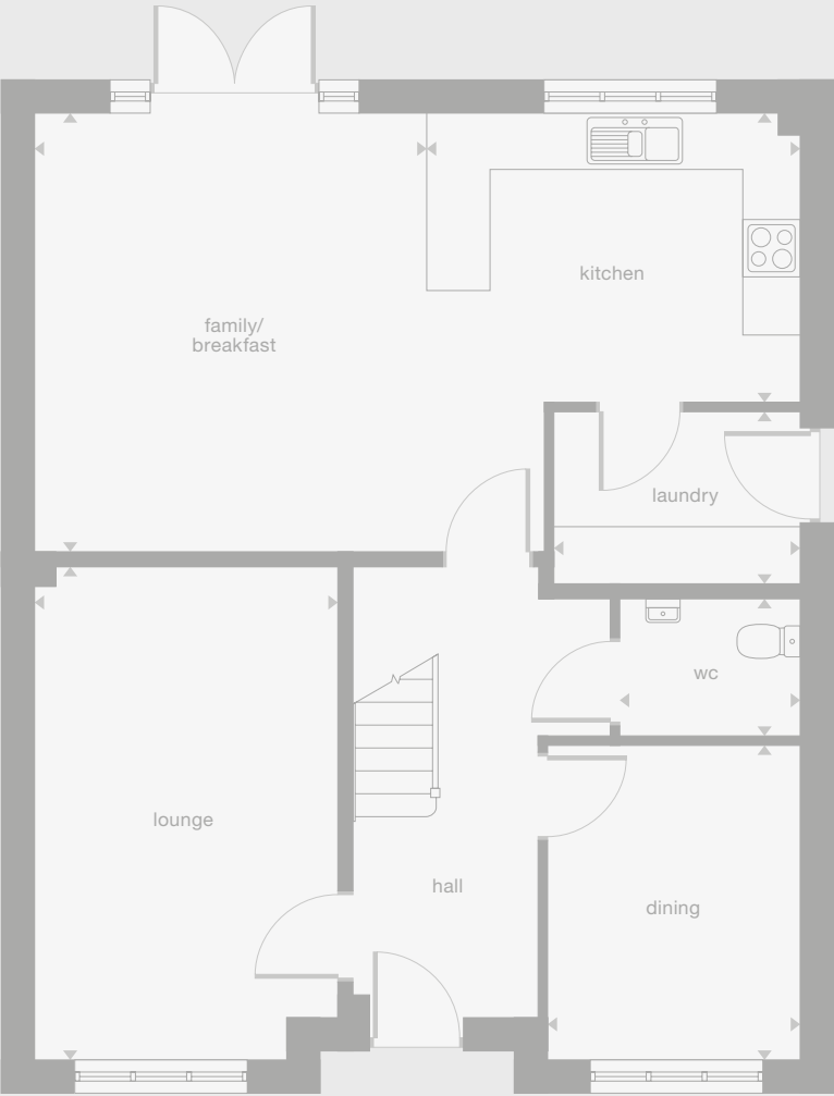
Ground Floor
